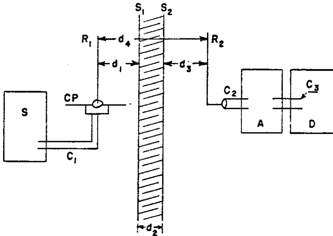
FIGURE 3.—Attenuation measurement high impedance electric field.
