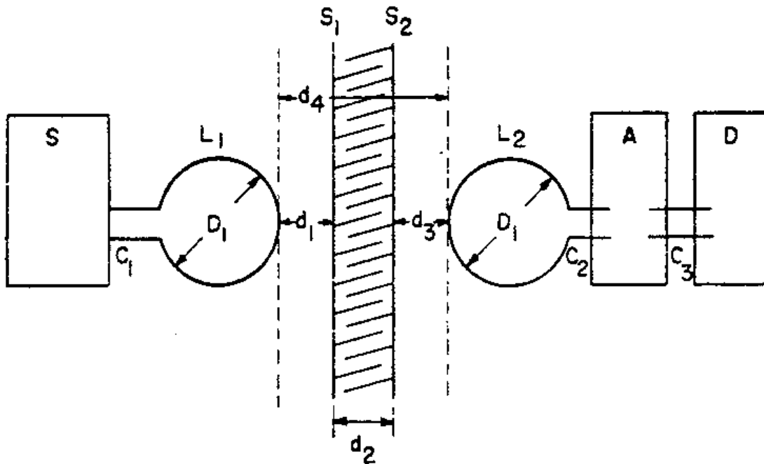
FIGURE 1.—Attenuation measurement low impedance magnetic field.
