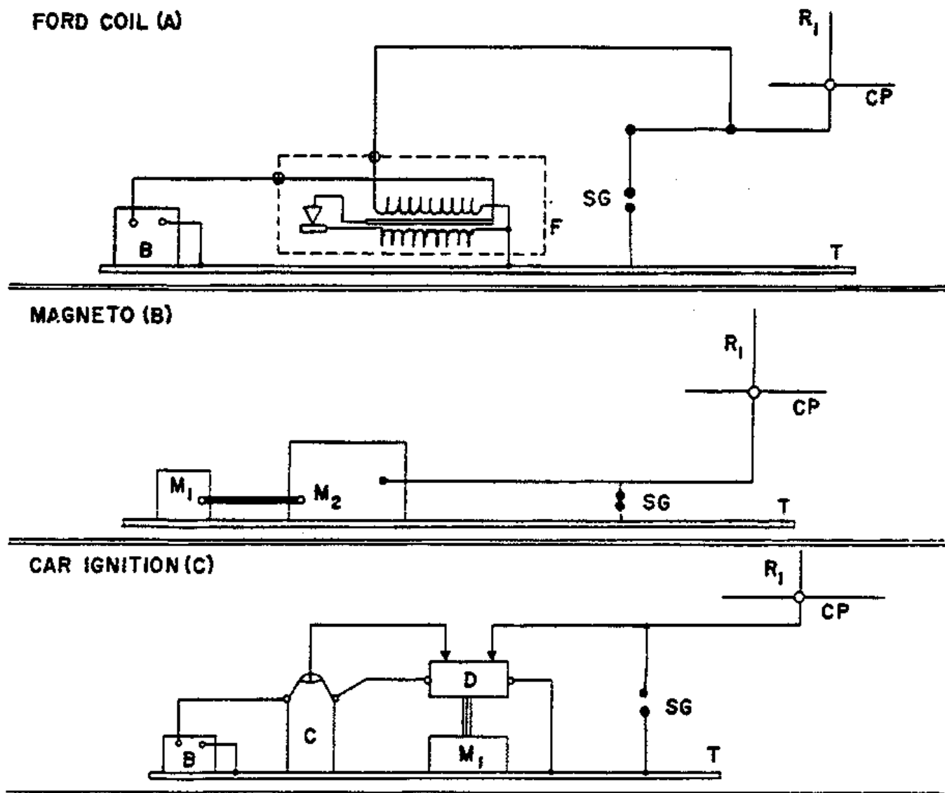
FIGURE 4.—Source for intense peak power electric field.
