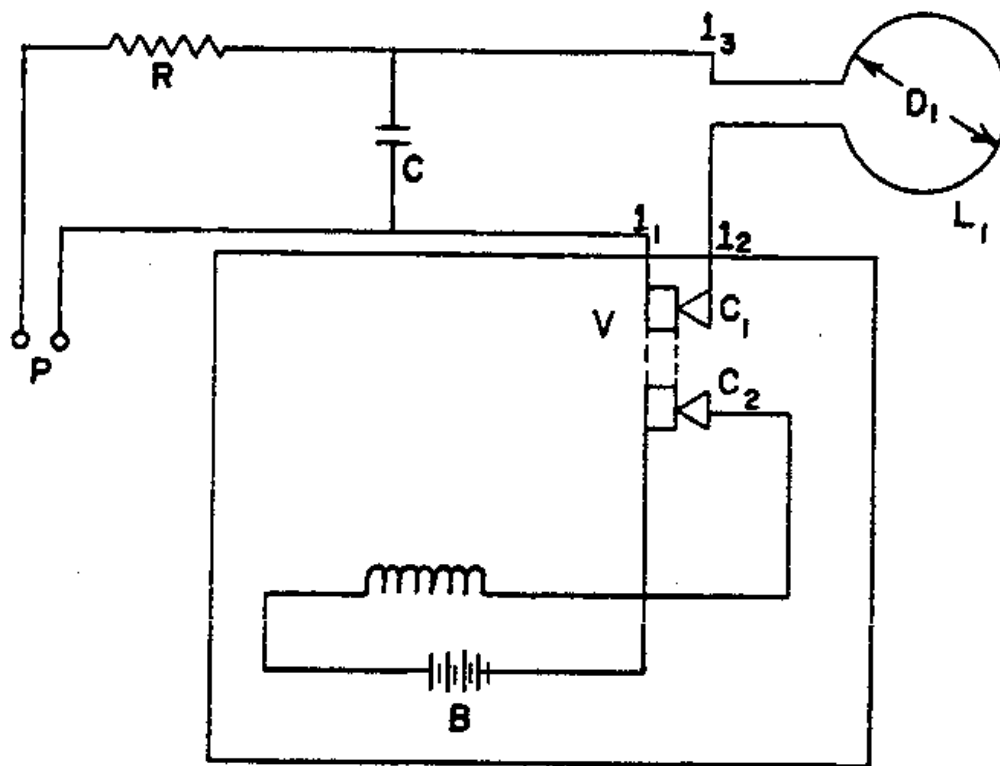
FIGURE 2. —Source of intense peak power magnetic field.
