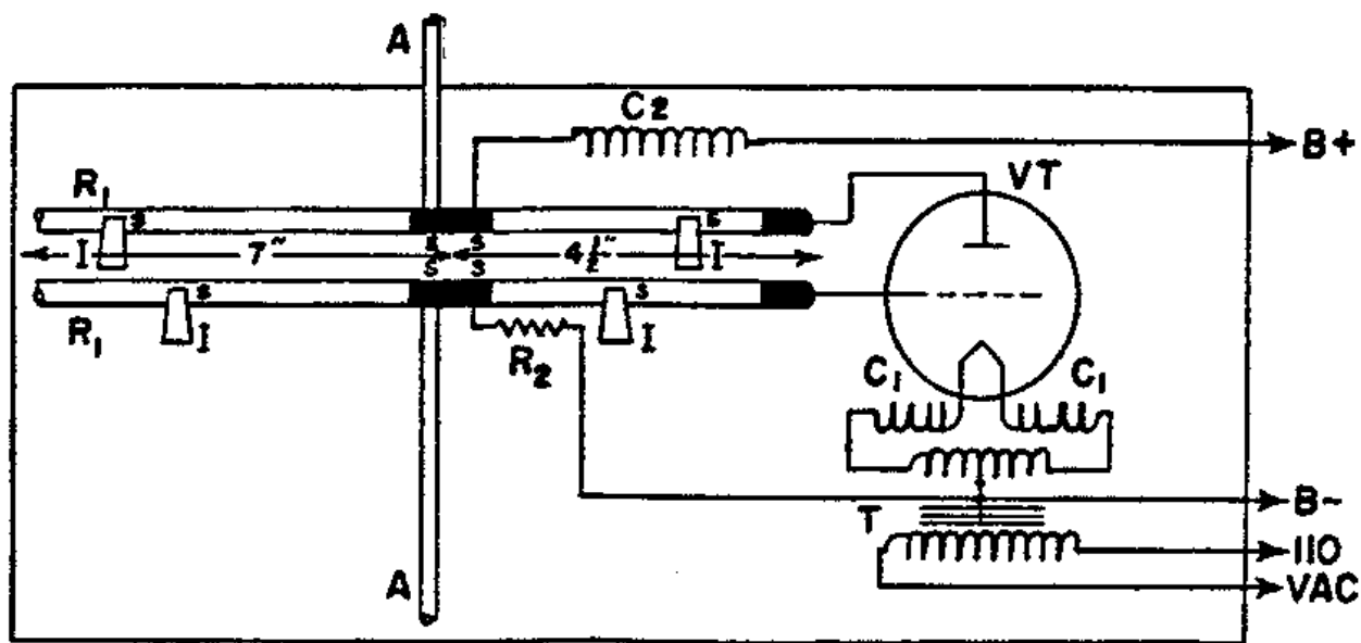
FIGURE 6.—Signal source for plane waves at 400 mc.
