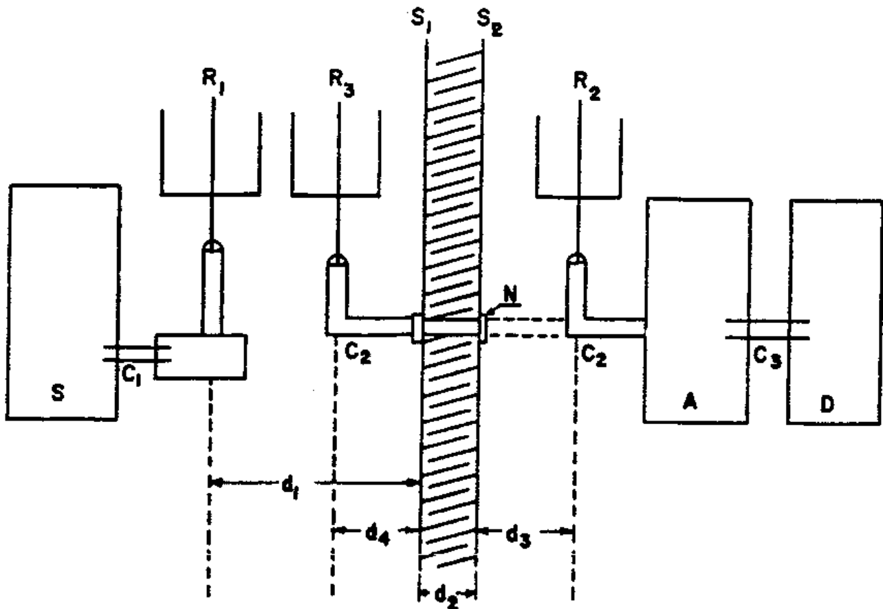
FIGURE 5.—Attenuation test for plane waves (wave impedance = 377 ohms).
